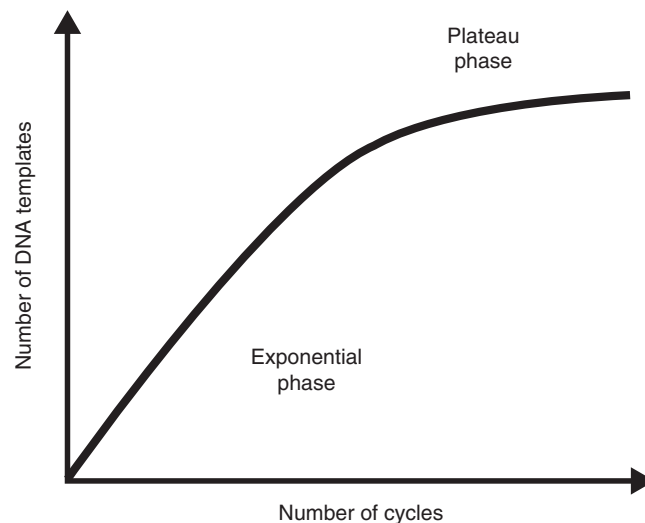
Fig. 24.2 Plateau effect in PCR
