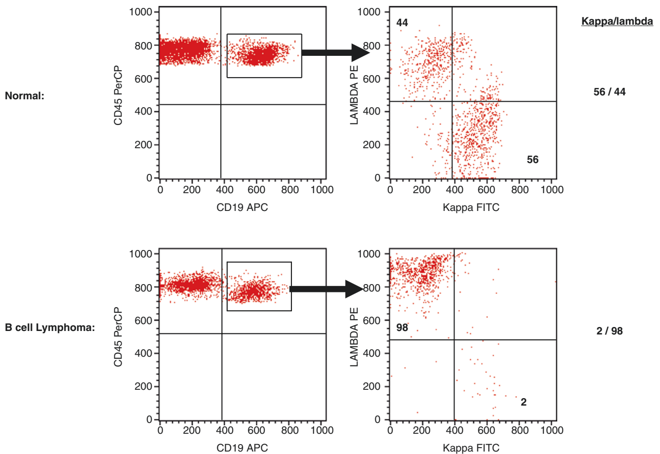
Fig. 22.9 B cell clonality. The ratio of kappa and lambda light chain expressing B cells can be used to determine clonality of B lymphocytes
