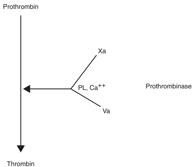
Fig. 10.2 The prothrombinase assembly for thrombin generation
